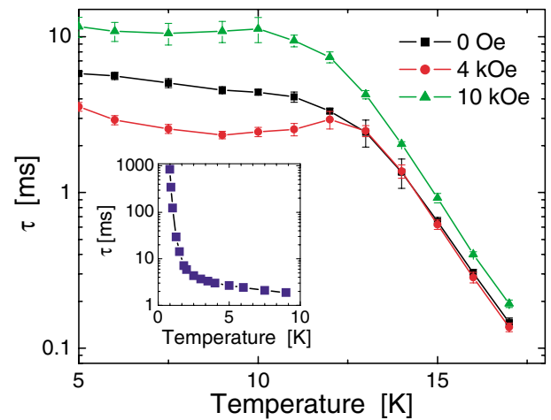
FIG. 3 (color online). The characteristic relaxation time, \tau , as a function of temperature at various applied fields. Inset: \tau(T) at H = 0 for a sample potted in epoxy down to T < 2 K [19].
