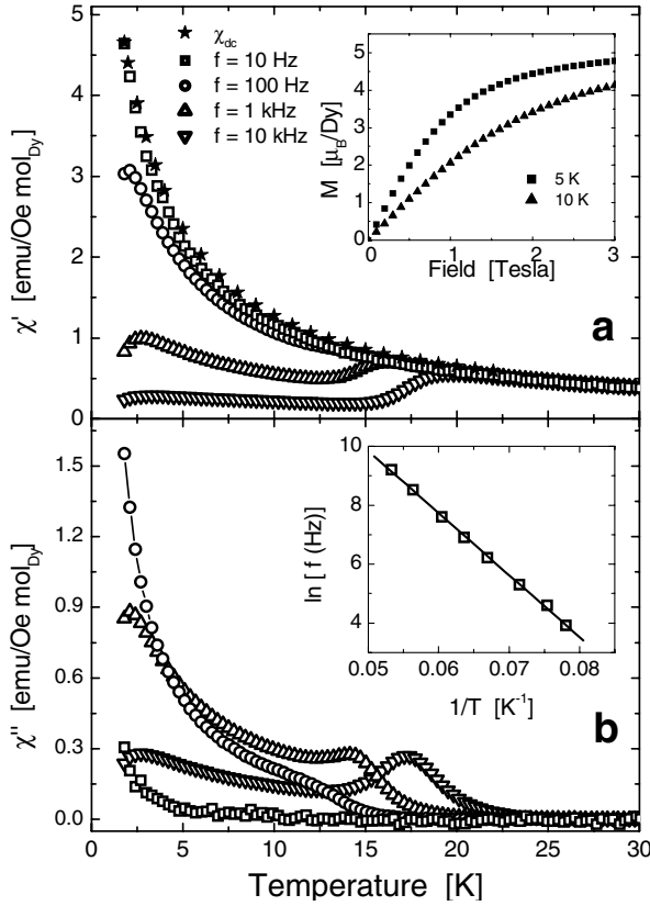
FIG. 1. Temperature dependence of the magnetic susceptibility for H = 0 . (a) The dc susceptibility and real part of the ac susceptibility ( \chi' ). Inset: the dc magnetization versus applied field. (b) The imaginary part of the ac susceptibility ( \chi'' ). Inset: the measurement frequency versus inverse freezing temperature, fit to an Arrhenius law.
