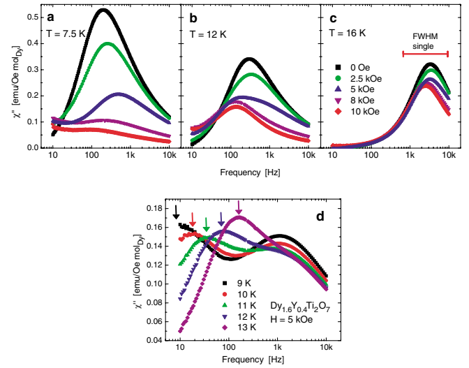
FIG. 2 (color online). (a)–(c) The frequency dependence of the imaginary part of the ac susceptibility ( \chi'' ). The peak magnitude decreases monotonically with increasing field. The bar in the 16 K plot shows the full width at half maximum of the theoretical response of a system with a single relaxation time. (d) Similar data at H = 5 kOe in a sample diluted with 20% Y on the Dy site. The data show two distinct peaks, confirming the existence of two separate relaxation processes. The colored arrows indicate the temperature dependent (classical relaxation) peak which moves down in frequency with decreasing temperature.
