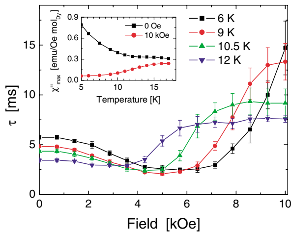
FIG. 4 (color online). The field dependence of the characteristic spin relaxation time, \tau . Inset: the magnitude of the peak in \chi''(f) as a function of temperature at H = 0 and 10 kOe.
